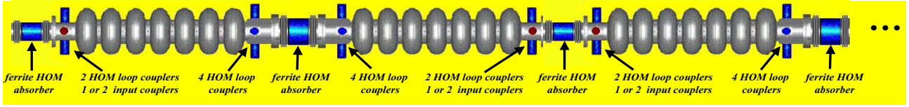
Figure 3: Sketch of the cavity string for the Cornell ERL main linac.
