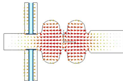
Figure 2: 2-cell cavity with twin RF input couplers.
