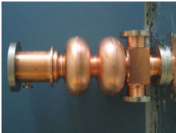
Figure 6: 2-cell injector prototype copper cavity.
