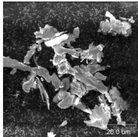
Figure 4: Copper particles generated from RF fingers.
