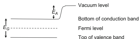
Fig. 2. The energy levels of a simple semiconductor [33].
