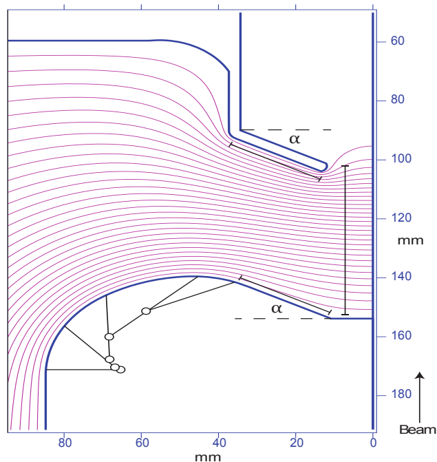
Figure 1: Gun geometry parameters for optimization. Each line represents a parameter varied by the optimizer. The geometry shown is that on the optimal front which has simultaneously minimum focal length and maximum field on the non-active region of the cathode electrode.
