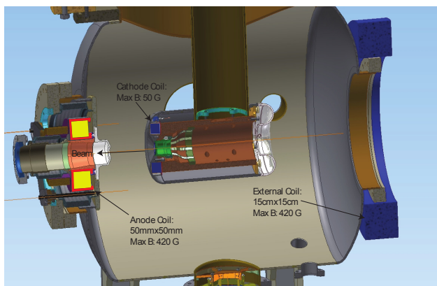
Figure 3: CAD drawing of gun assembly, showing anode coil, and two bucking coil options: embedded solenoid (within cathode) and external solenoid (both shown in blue).
