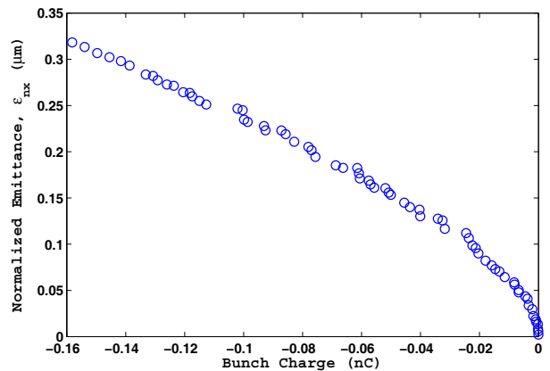
Figure 2: Full-beamline emittance optimization for varied bunch charges.
