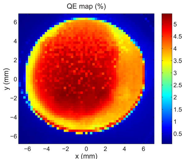
FIG. 3. (Color online) QE map of the photocathode inside the dc gun.
