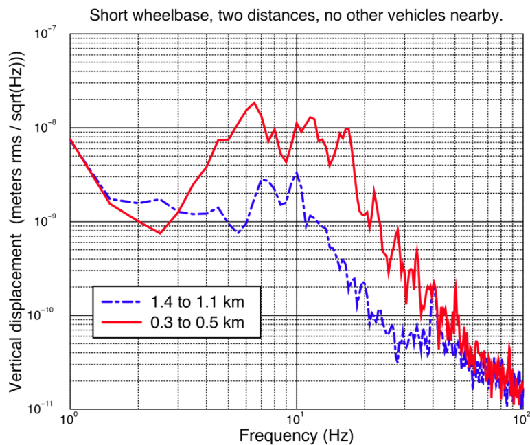
Figure 2.10.13: Seismic signal from a truck on the highway near LIGO site at Hanford Washington. Signal measured in test pits near the LIGO interferometer.
