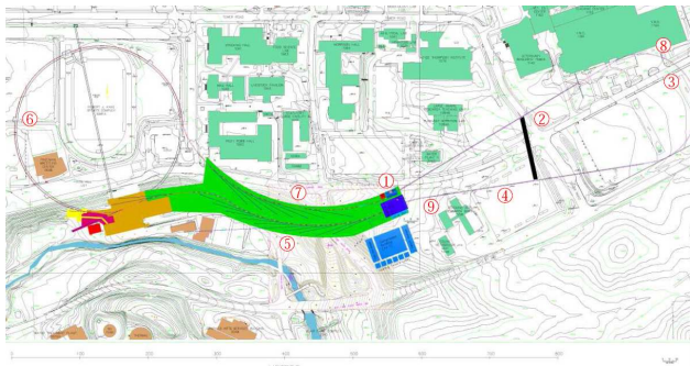
Figure 1: Current layout of Cornell's x-ray ERL.
