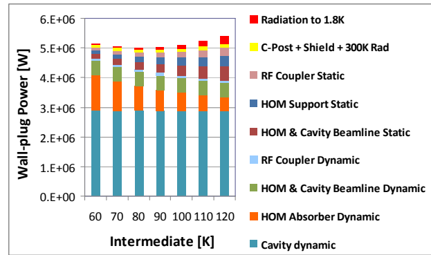
Figure 4: ANSYS modeled wall-plug refrigeration power for a 64-module ERL linac as a function of the intermediate intercept temperature.
