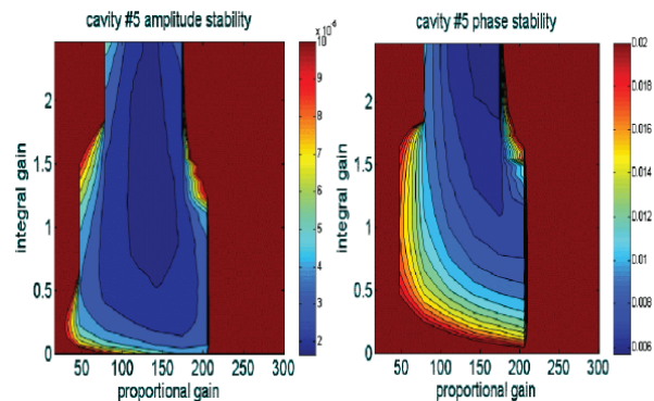
Figure 10: Integral and proportional gain scan to optimize the gains used in the field control loop. Left: Amplitude stability (blue: \sigma_A/A < 2 \times 10^{-5} ). Right: Phase stability (blue: \sigma_p < 0.01^\circ ).
