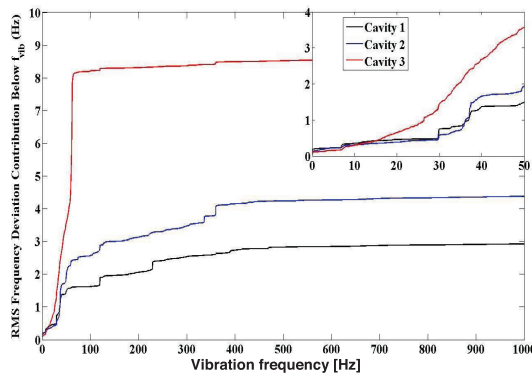
Figure 12: The integrated microphonic spectra for three different cavities in the ERL injector module.
