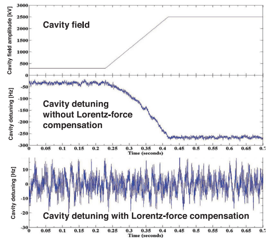
Figure 13: Top: The cavity field is ramped up to 2.5 MV in 0.2 seconds. Middle: Lorentz-force detuning without active compensation. The Lorentz-force detuning coefficient is 2 \text{ Hz}/(\text{MV}/\text{m})^2 . Bottom: Cavity detuning during field ramp up with active detuning compensation.
