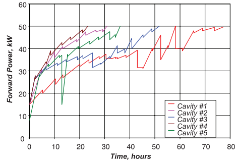
Figure 6: Input coupler processing under full reflection (cavity detuned) up to 50 kW. Shown is the maximum forward power per twin-coupler vs. of processing time (pulsed operation with 2 ms pulse length and 20 ms repetition rate).
