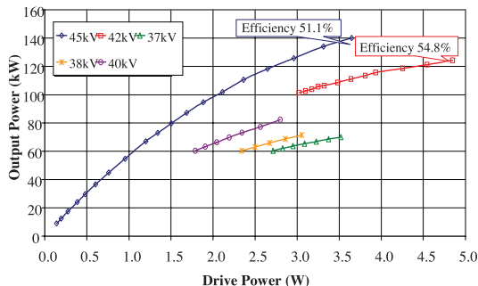
Figure 5: Transfer curve of the ERL injector klystron.
