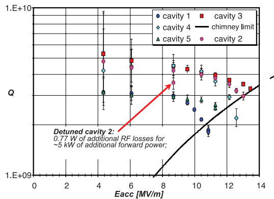
Figure 8: Intrinsic quality factor of the five 2-cell injector SRF cavities as a function of accelerating field gradient at 2K. Also show is the 1 W/cm 2 heat flux limit for the LHe in the chimney connecting the LHe tank around the cavity to the 2K-2 phase LHe supply line.
