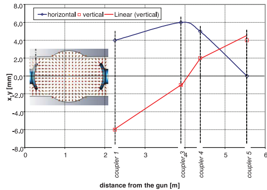
Figure 7: Orbit of a very low energy (250 keV) electron beam in the injector cryomodule as estimated by measuring transverse kicks by the RF fields in the input coupler regions. The RF field is excited by a forward power of up to 1 kW with strongly detuned cavities. The resulting electric RF field has a quadrupole like pattern, as shown on the left. By measuring magnitude and direction of the kick to the beam at a given forward power, the beam position in the coupler region can be determined.
