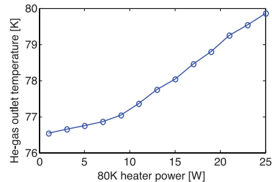
Figure 9: Measured temperature increase of the 80K He outlet gas vs. HOM heater power during calibration.
