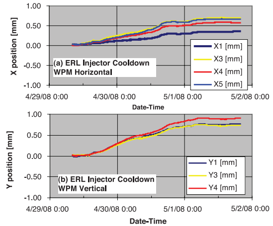
Figure 4: WPM data during cool-down of the injector module. Top: Horizontal position of WPM blocks on cavities 1, 3, 4, and 5. Bottom: Vertical position of WPM blocks on cavities 1, 3, and 4. WPM #2 is not functional.
