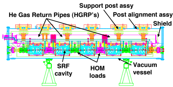
Figure 3: Longitudinal cross-section of the ERL injector module with 5 SRF cavities with HOM beam line absorbers in between. The module is longitudinally separated in three sections, each supported and aligned independently.
