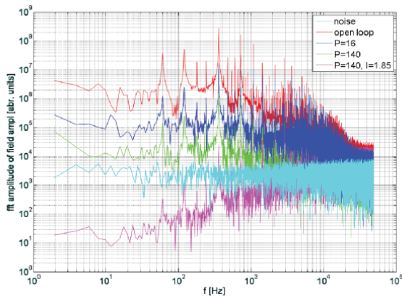
Figure 11: FFT amplitude spectrum of the cavity RF field amplitude for different gain settings. Also shown is the noise spectrum without input connected to the 50 MHz, 16 bit ADC used in sampling the RF field, corresponding to an integrated rms fluctuation of 0.1 bits for f < 50 kHz.
