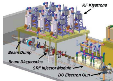
Figure 1: Layout of the ERL injector prototype.
