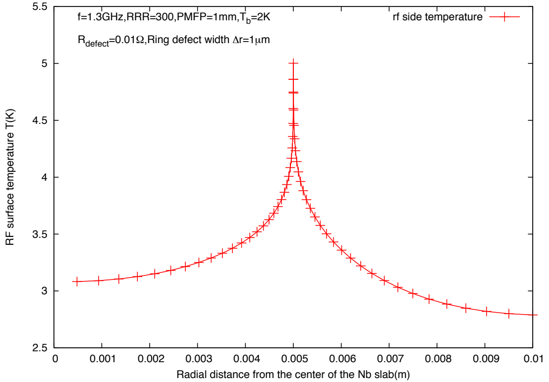
Figure 6.9: rf surface temperature distribution of a 5 mm ring-type defect with 1\ \mu\text{m} width. The modeled niobium plate has a radius of 10 mm. The rf frequency is 1.3 GHz, RRR = 300, phonon mean free path = 1 mm, bath temperature = 2 K, magnetic field = 500 Oe and the normal conducting defect resistance is 10\ \text{m}\Omega .
