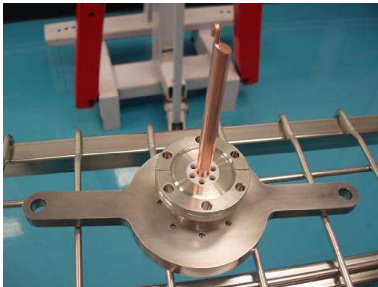
Figure 3.29: Completed rf input coupler for the TE cavities after final assembly.
