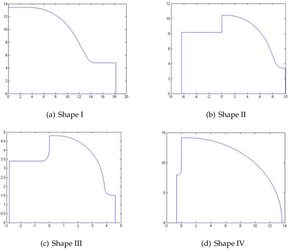
Figure 3.7: Four basic shapes of TE sample host cavities.
