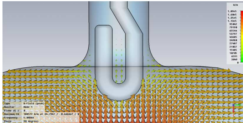
Figure 3.14: Magnetic field distribution near a “Saclay” style loop coupler calculated by MWS.
