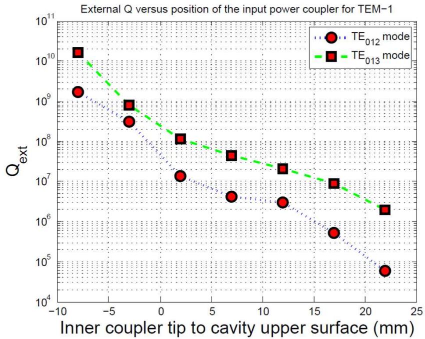
Figure 3.16: Q_{ext} dependence on coupler penetration depth into the cavity.
