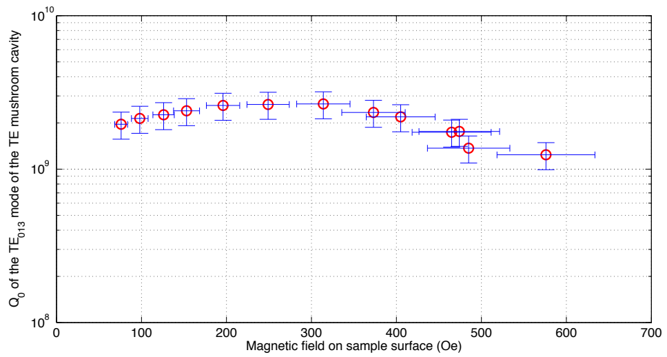
Figure 4.6: TE mushroom cavity quality factor Q_0 of mode TE 013 versus maximum magnetic field on the sample. The uncertainty in measured field is \pm 10\% and the uncertainty in measured Q_0 is \pm 20\% .
