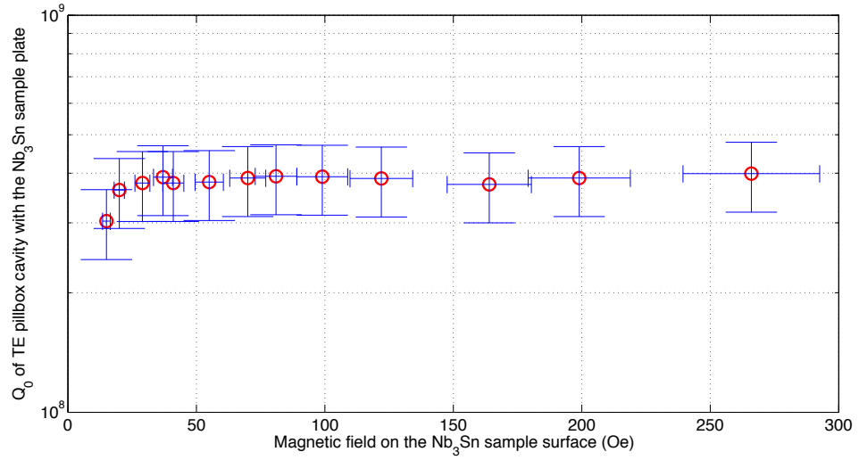
Figure 4.15: Measured quality factor Q_0 vs maximum magnetic field on the \text{Nb}_3\text{Sn} sample plate as measured in the TE pillbox cavity at 1.6 K. The uncertainty in measured field is \pm 10\% and the uncertainty in measured Q_0 is \pm 20\% .
