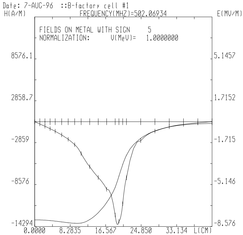
Figure 10. Surface fields for the fundamental mode. Metafile BB1_SLR04.MTF
