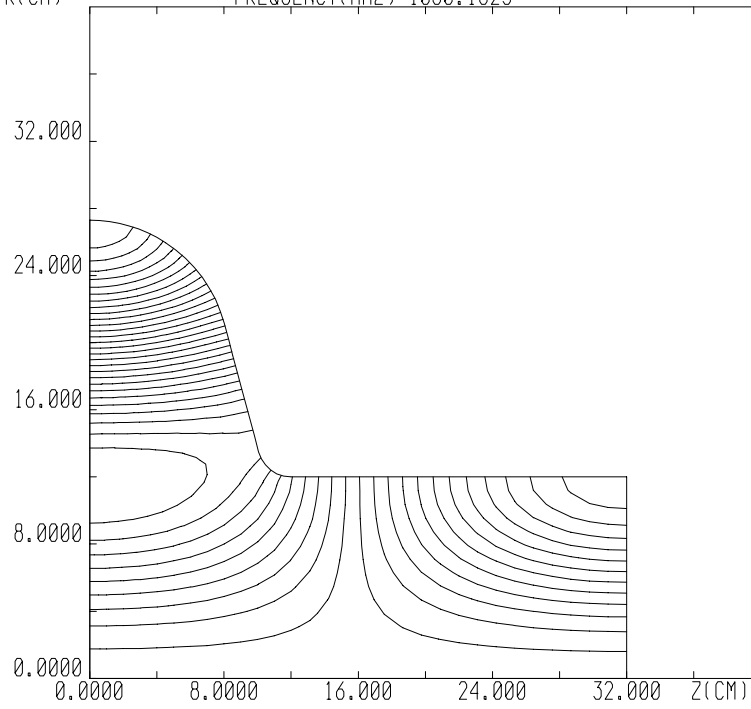
Figure 8. Force lines for one of the HOMs. Metafile BB1_SLR02.MTF
