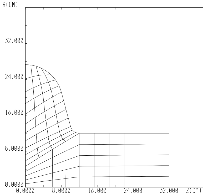
Figure 4. The mesh for the BB1 cavity. File BB1_GEN01.MTF
