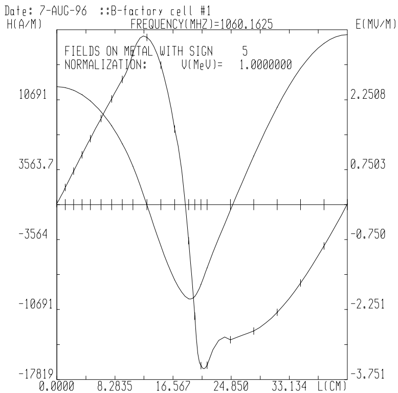
Figure 11. Surface fields for one of the HOMs. Metafile BB1_SLR06.MTF
