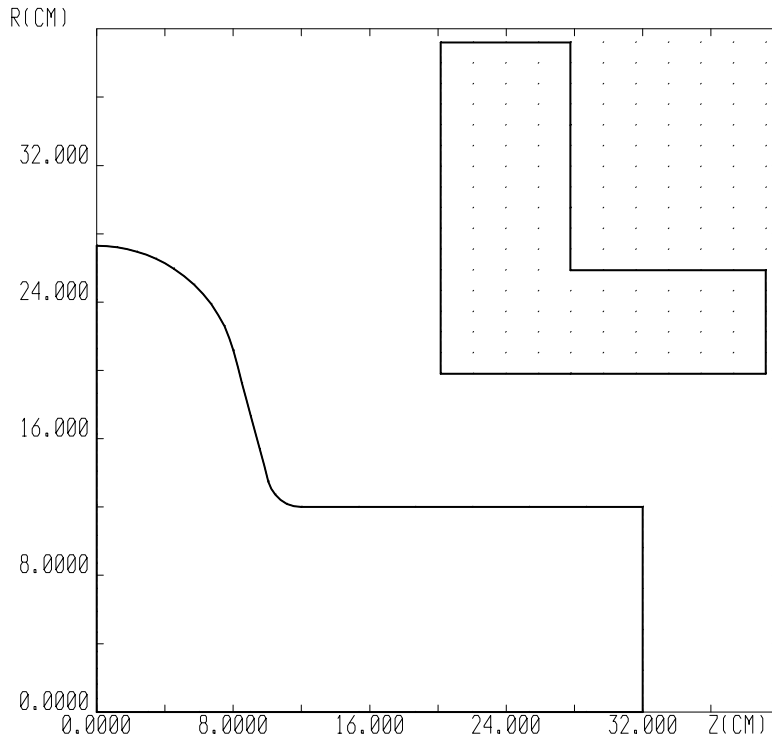
Figure 2. The BB1 geometry. File BB1_ING01.MTF
