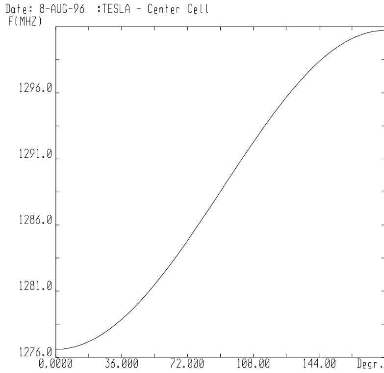
Figure 13. A dispersion curve for the TeSLA structure. Metafile TESLA_SLR01.MTF
