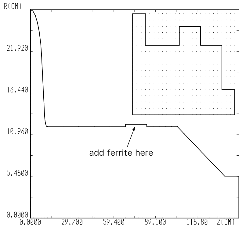
Figure 14. Cavity Geometry
