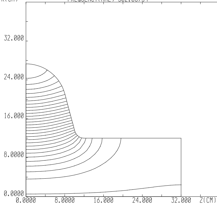
Figure 7. Force lines for the fundamental mode. Metafile BB1_SLR01.MTF
